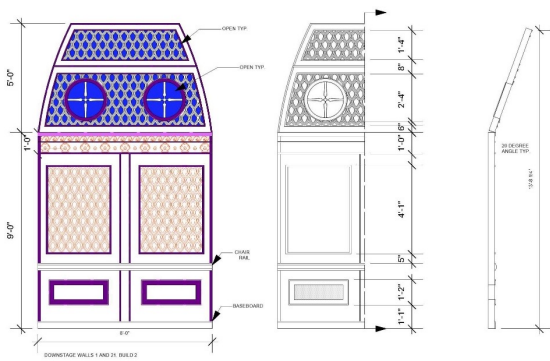
CONNECTING WALLS 1 AND 21, BUILD 2
